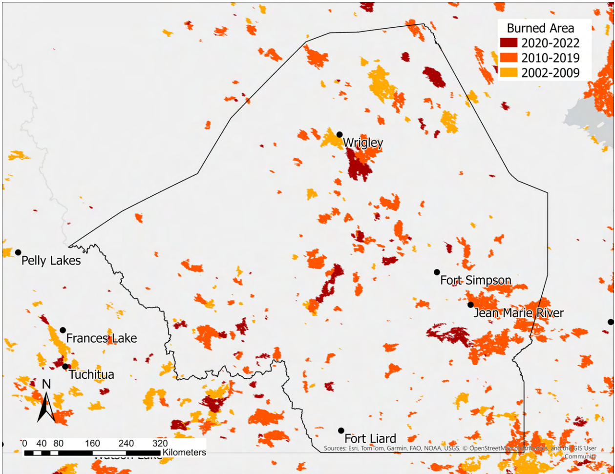
Dehcho Region burned area between 2002 and 2022
