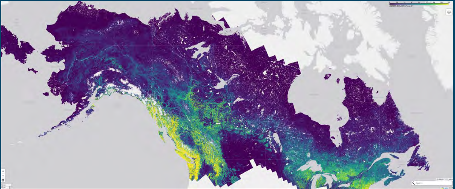
Aboveground biomass ( \text{Mg ha}^{-1} ) for boreal forest estimated from ICESat-2 imagery
