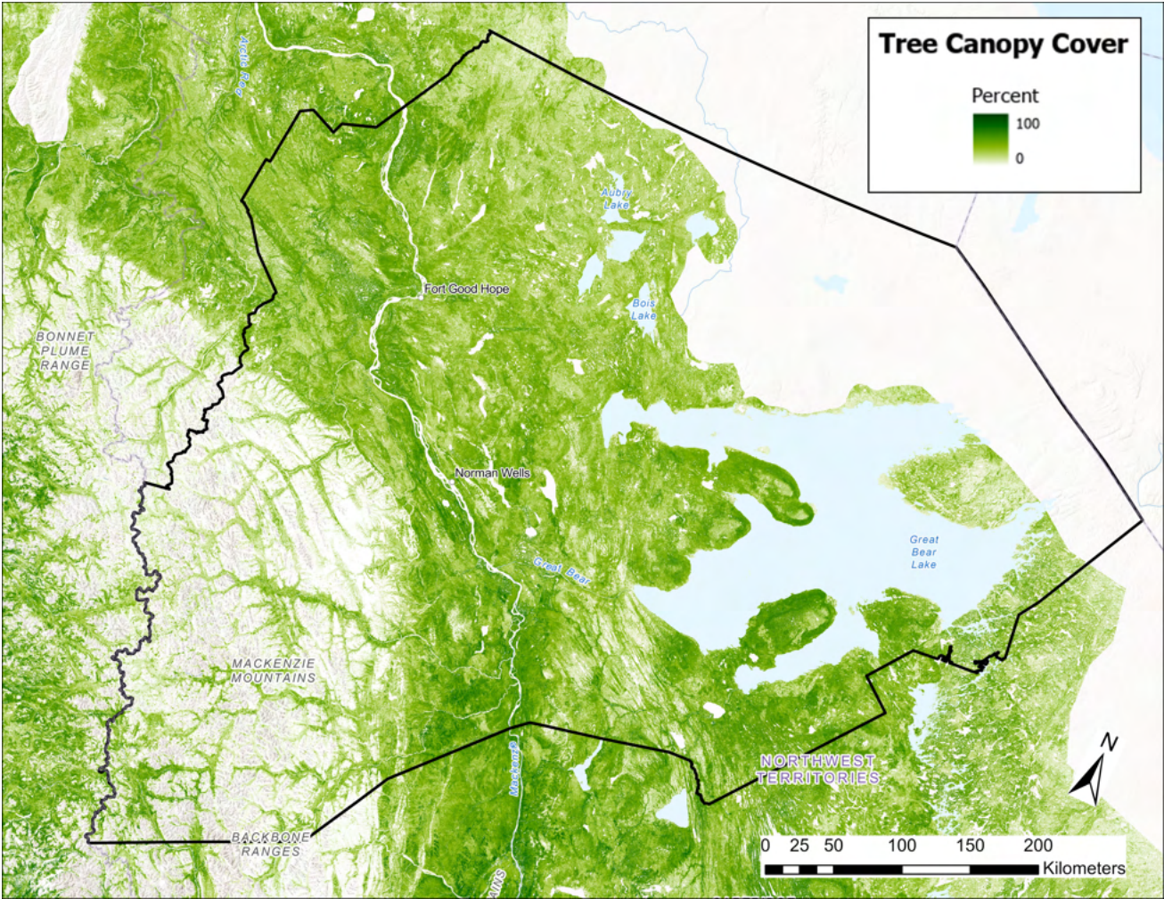
Sahtu Region Tree Canopy Cover in 2020
