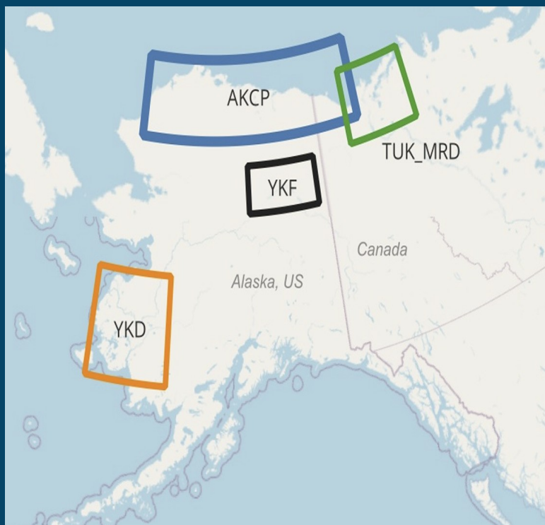
Left: Study regions for weekly surface water occurrence. "AKCP" = Alaskan Coastal Plain, "YKF" = Yukon Flats, "YKD" = Yukon-Kuskokwim Delta, "TUK_MRD" = Tuktoyaktuk Peninsula and Mackenzie River Delta.
