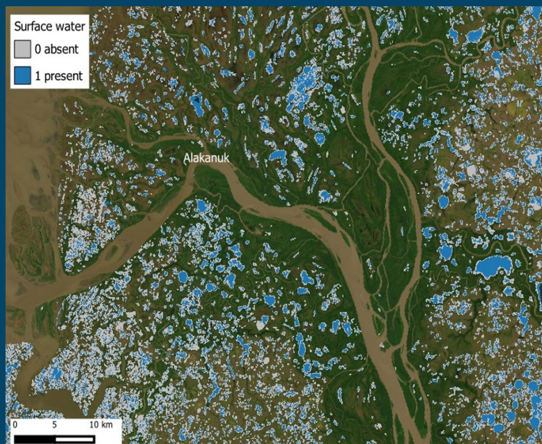
Right: Occurrence of surface water in Yukon-Kuskokwim Delta near Alakanuk, Alaska, during week 35 of 2017 (2017-09-03 to 2017-09-09). Surface water presence-absence was estimated from Sentinel-2 imagery for pixels with a lake-and-pond analysis mask.
