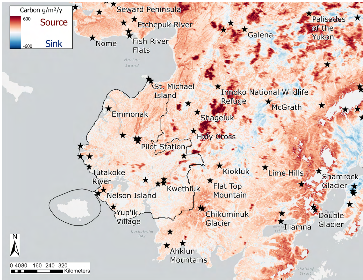
Yukon-Kuskokwin Delta \text{CO}_2 Fluxes showing the Net Ecosystem Exchange and Net Ecosystem Fire from 2001-2020
